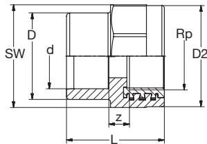
BR PVC-U-Rotguss/Messing/LFB Übergang IG-zy1 grau BR PVC-U-Bronze/Brass/LFB Transition female-thread-cyl grey
