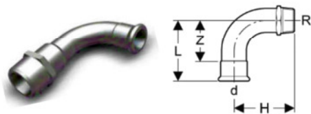
Adattatore 90° fil. maschio Bend adaptor 90° with male thread Übergangsbogen 90° A.G.
