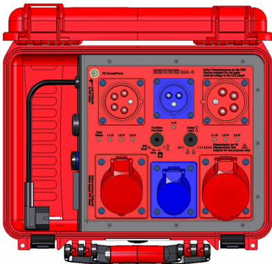
Abb. 6: BENNING MA 4
