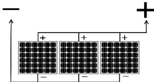
Parallel PV-Connector
