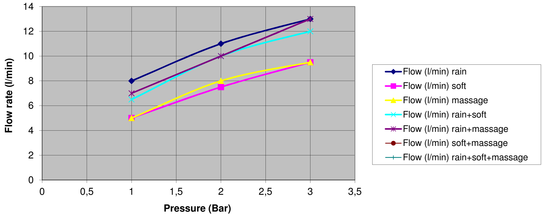
"LUNA 5 GETTI" Shower Flow
