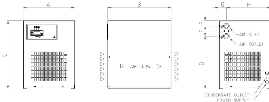
FRONT VIEW
