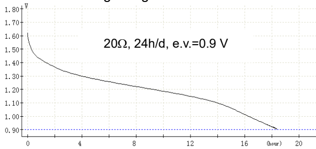
Chart 1. Discharge diagram
