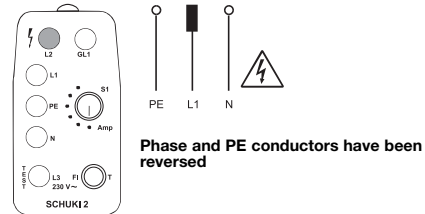
Figure 7: Lamp L2 only lights up. Touching the touch electrode has no effect.
