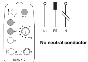
Figure 4: The lamps L1 and PE light up. GL1 lights up when the touch electrode is touched. You must observe the fault depicted in figure 5.
