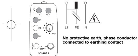
Figure 8: The lamps N , L1 and L2 light up. GL1 lights up when the touch electrode is touched.
