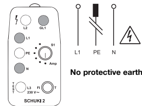
Figure 6: The lamps L1 and N light up. GL1 lights up when the touch electrode is touched.
