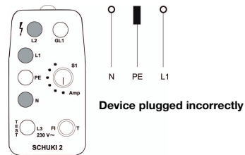
Figure 3: The lamps N , L1 and L2 light up. When the touch electrode is touched, the lamp GL1 does not light up. The phase conductor is not contacting the left-hand pin of the test device (viewed when device is inserted and faceplate visible); it cannot be tested. Rotate the Schuki 2 180° and re-insert.
