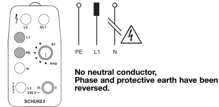
Figure 5: The lamps L1 and PE light up. Touching the touch electrode has no effect.
