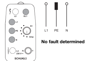
Figure 2: All lamps in the yellow area light up. The lamp GL1 must light up when the touch electrode is touched.
