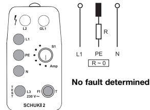
Figure 10: All lamps in the yellow area light up. In addition, the lamp L3 lights up when the button T is pressed. The lamps go out when the ELCB is tripped.
